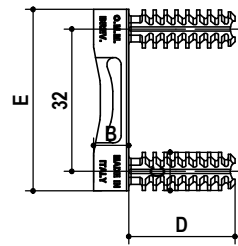
filetto mordente 2.9 chipboard head 2.9
